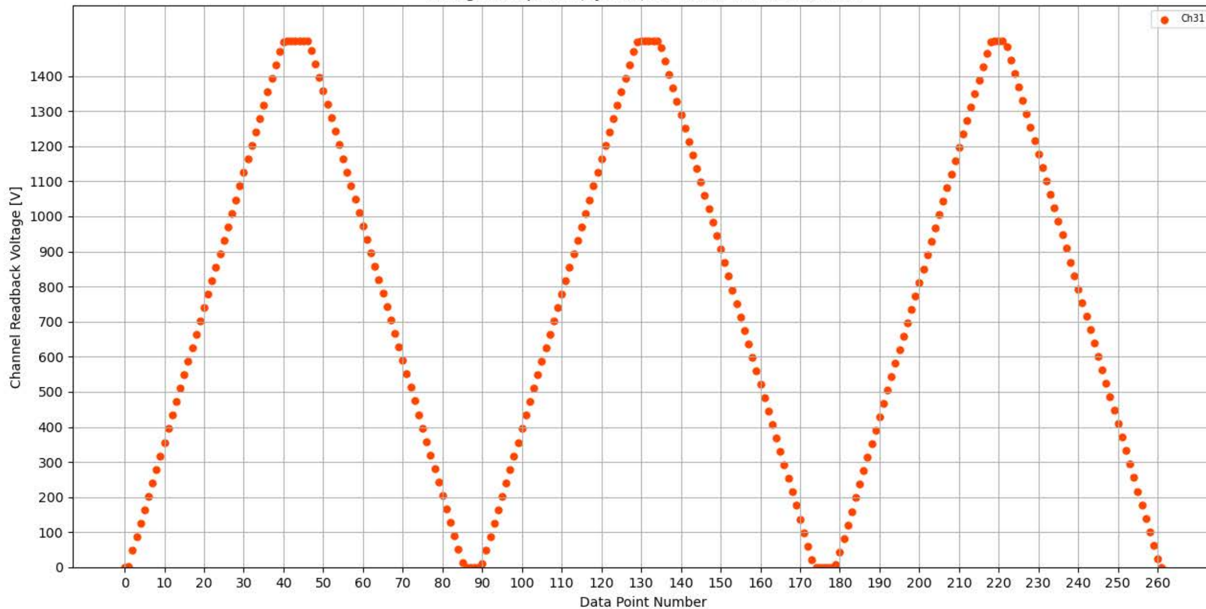
Voltage Ramp Test (Python) Bd #302, Slot #4, Ch #31
