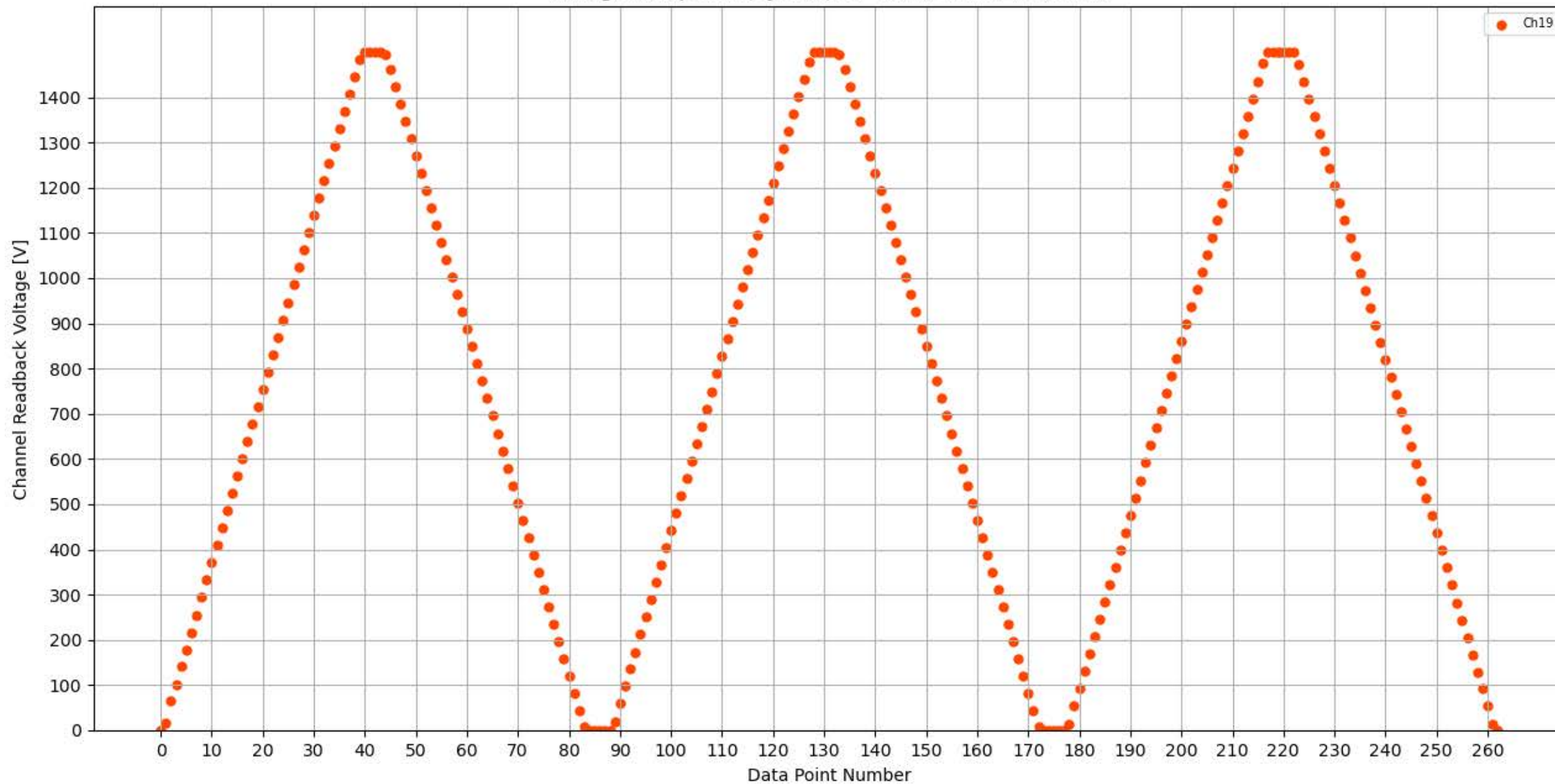
Voltage Ramp Test (Python) Bd #302, Slot #4, Ch #19
