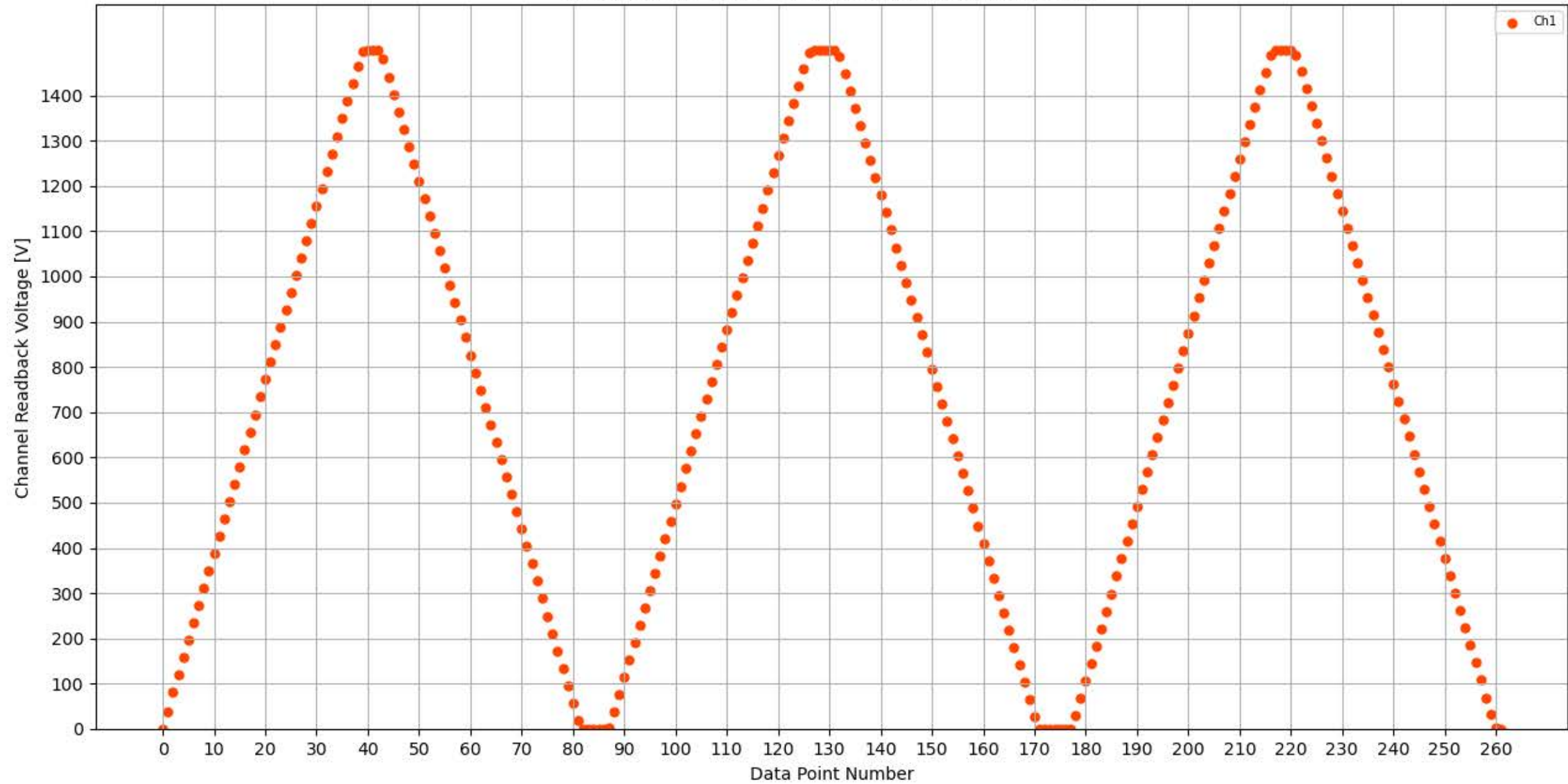
Voltage Ramp Test (Python) Bd #302, Slot #4, Ch #1
