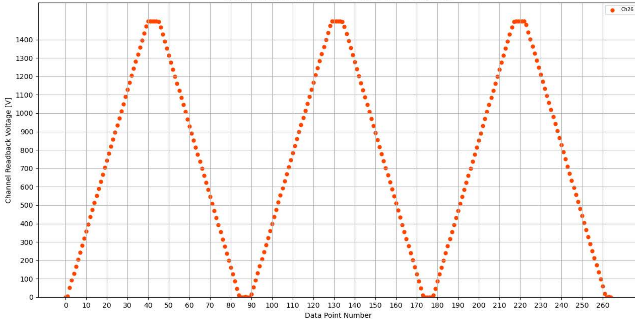
Voltage Ramp Test (Python) Bd #302, Slot #4, Ch #26
