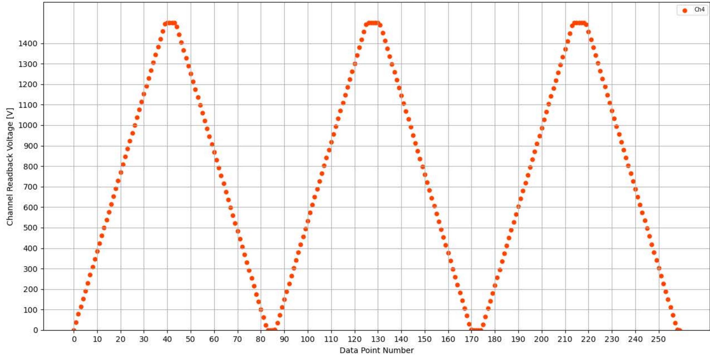
Voltage Ramp Test (Python) Bd #302, Slot #4, Ch #4
