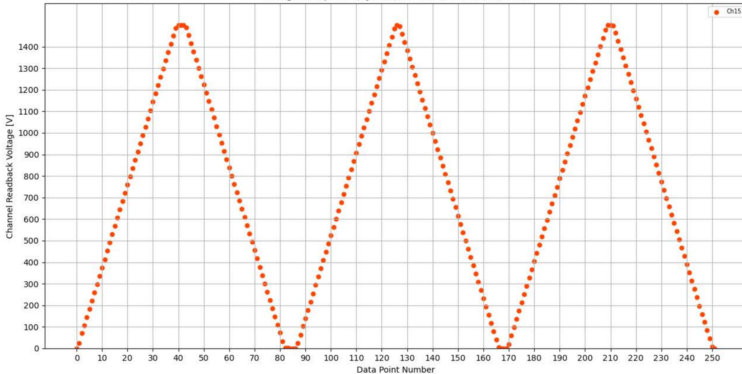
Voltage Ramp Test (Python) Bd #302, Slot #4, Ch #15
