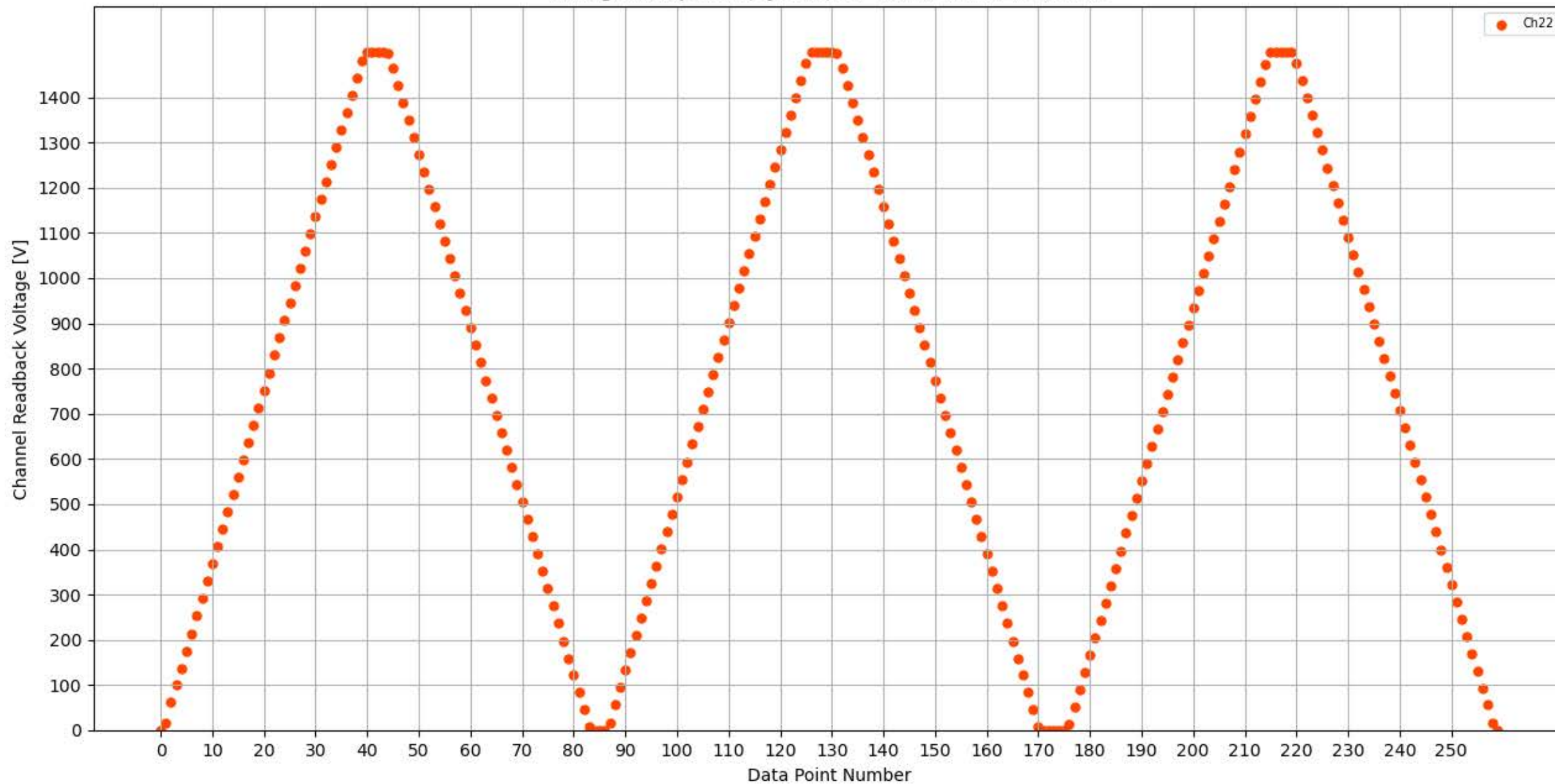
Voltage Ramp Test (Python) Bd #302, Slot #4, Ch #22
