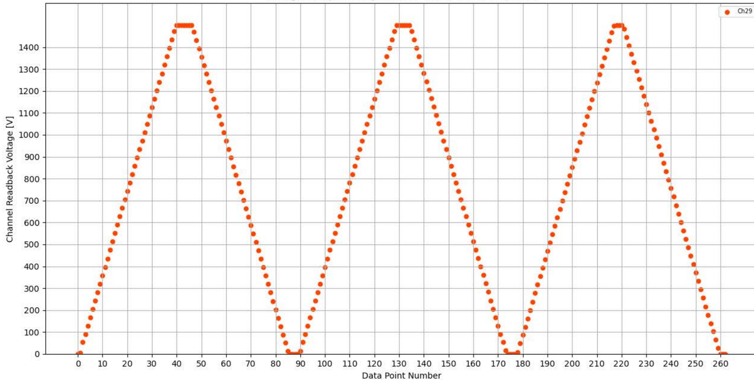
Voltage Ramp Test (Python) Bd #302, Slot #4, Ch #29
