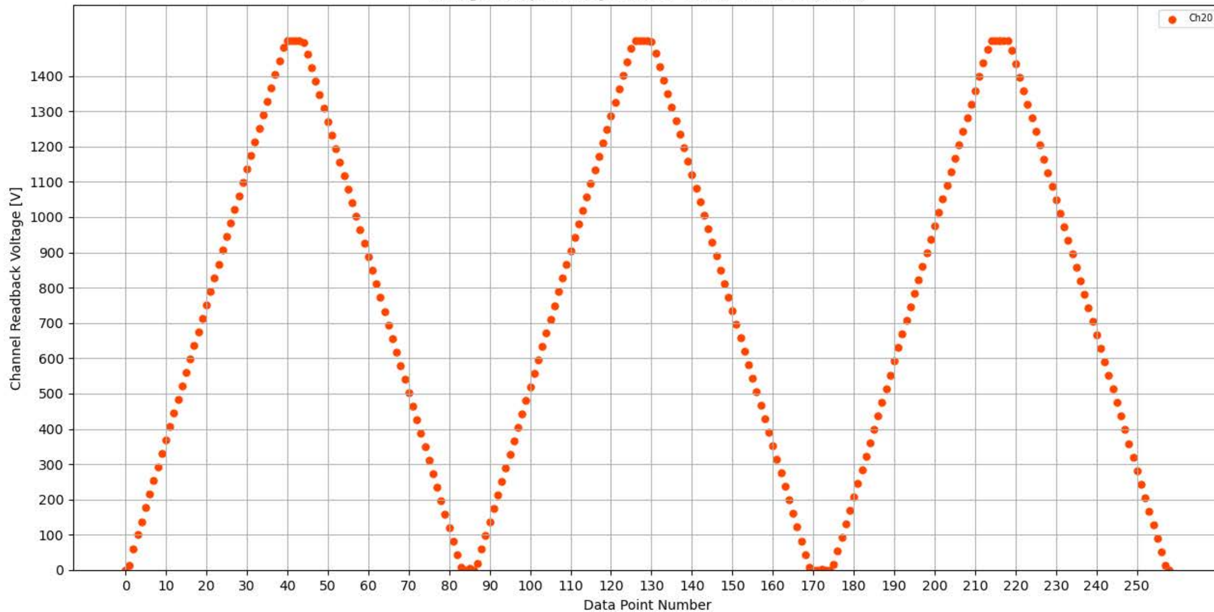
Voltage Ramp Test (Python) Bd #302, Slot #4, Ch #20
