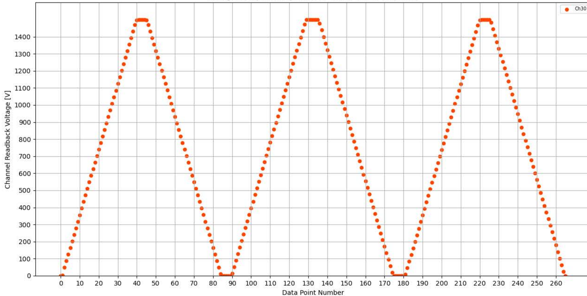
Voltage Ramp Test (Python) Bd #302, Slot #4, Ch #30
