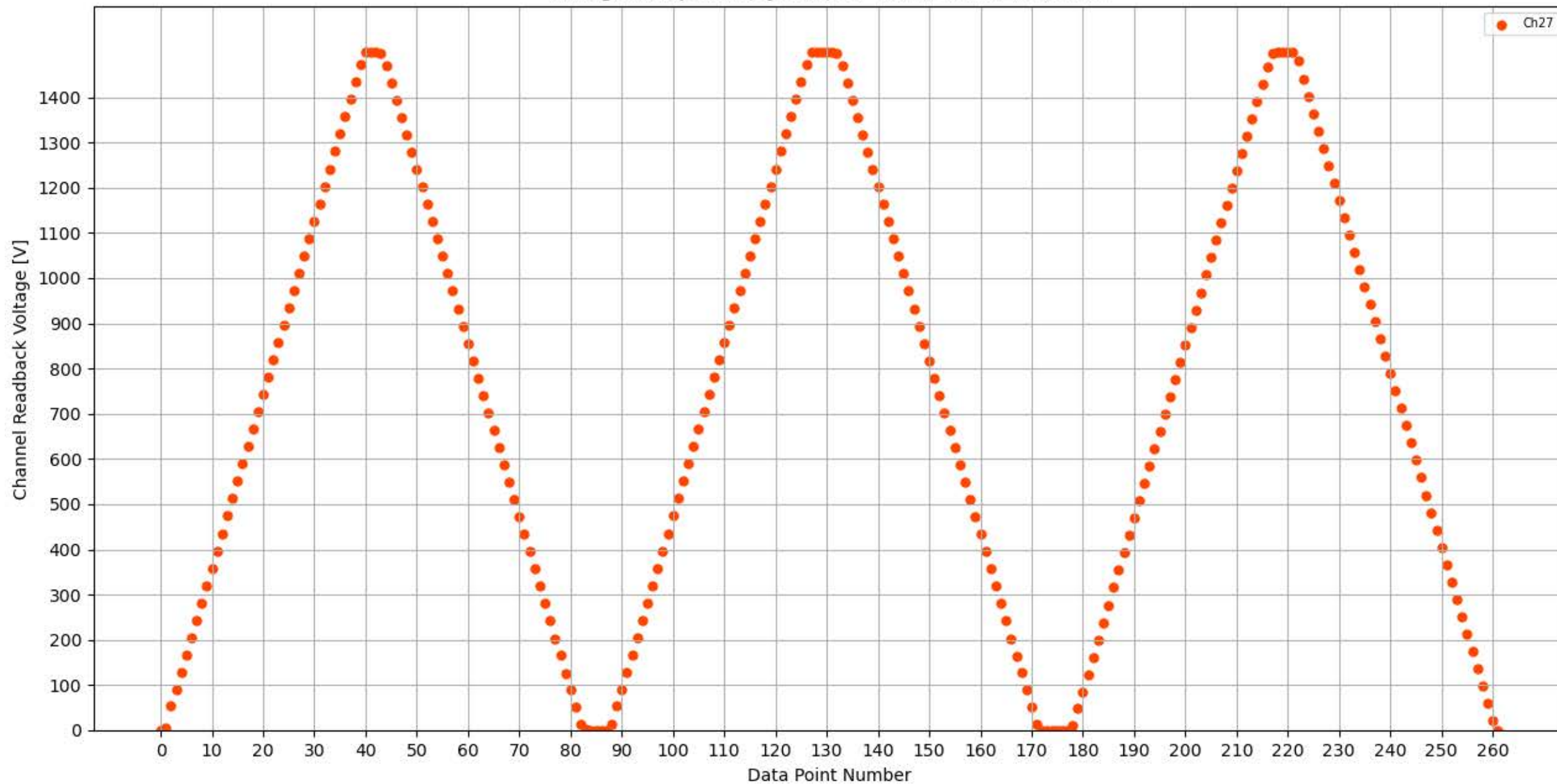
Voltage Ramp Test (Python) Bd #302, Slot #4, Ch #27
