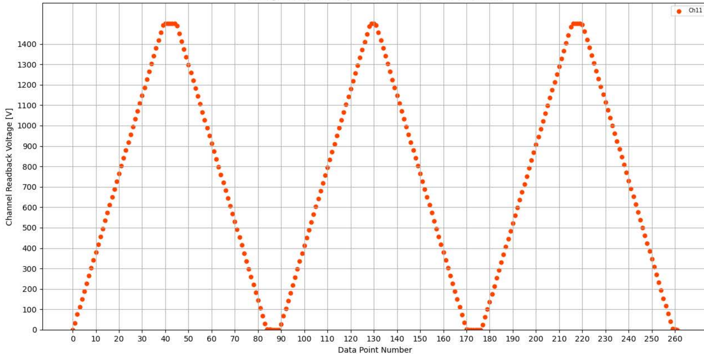
Voltage Ramp Test (Python) Bd #302, Slot #4, Ch #11
