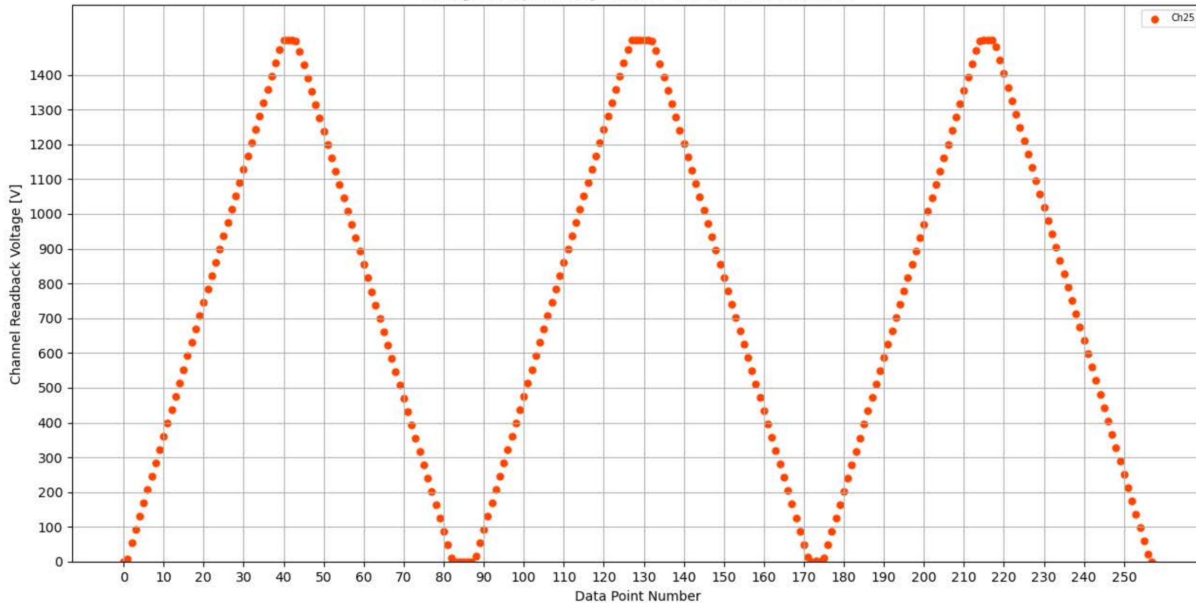
Voltage Ramp Test (Python) Bd #302, Slot #4, Ch #25
