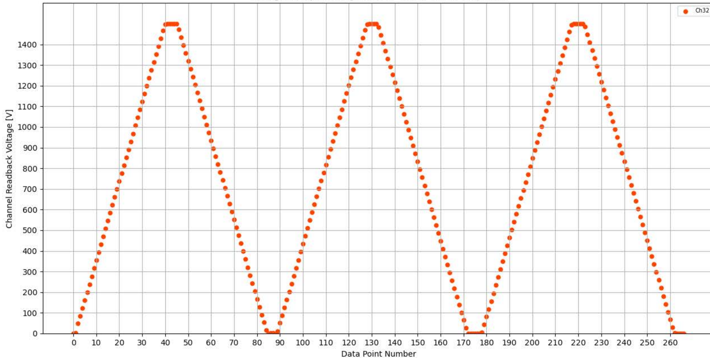
Voltage Ramp Test (Python) Bd #302, Slot #4, Ch #32
