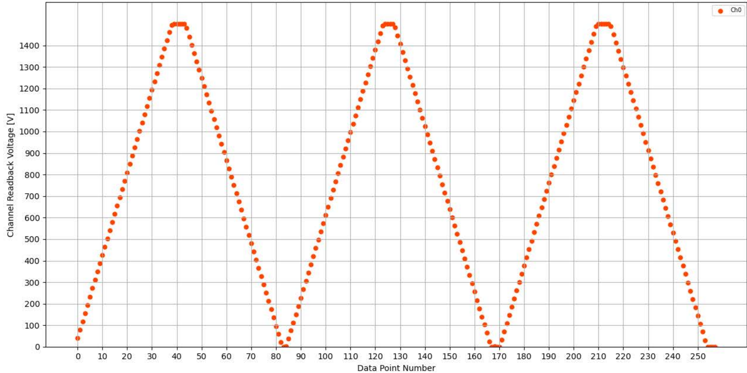
Voltage Ramp Test (Python) Bd #302, Slot #4, Ch #0
