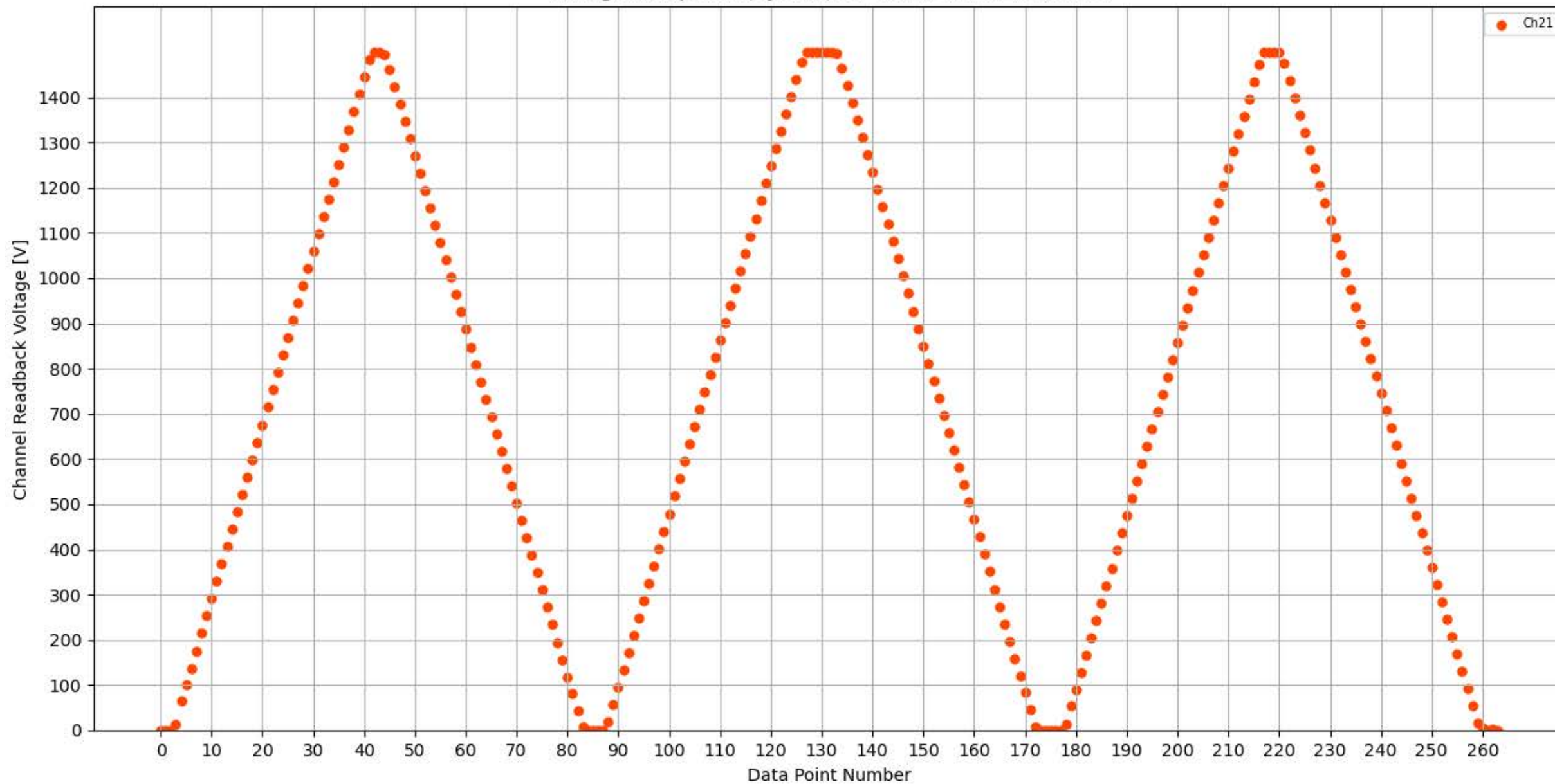
Voltage Ramp Test (Python) Bd #302, Slot #4, Ch #21
