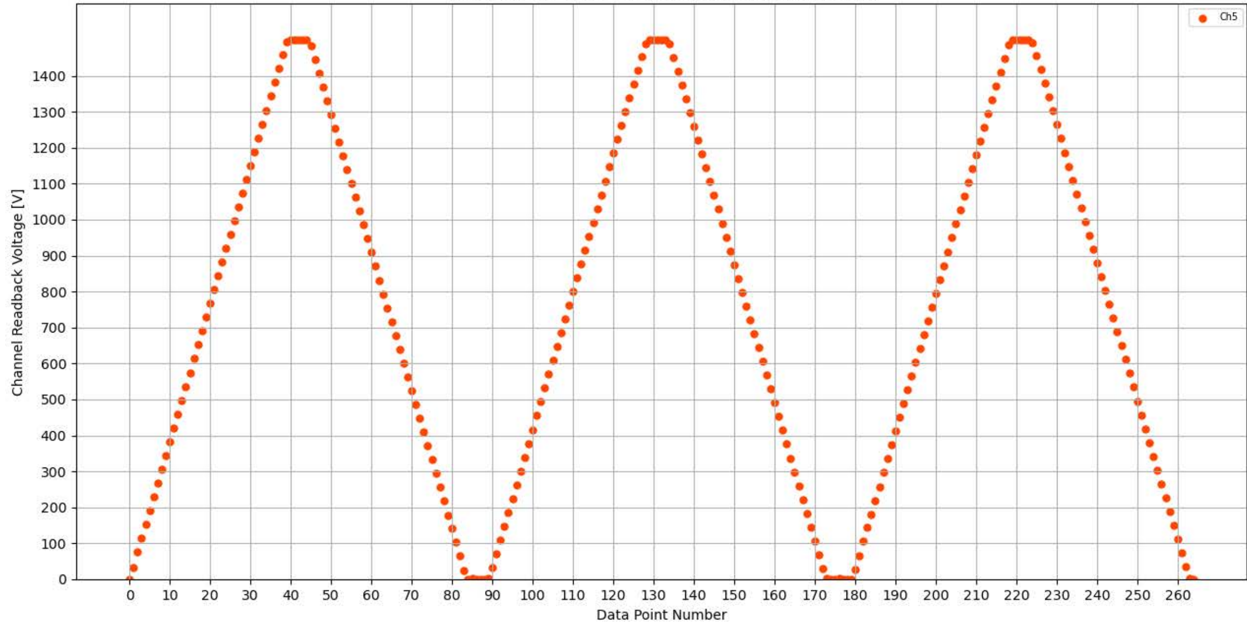
Voltage Ramp Test (Python) Bd #302, Slot #4, Ch #5
