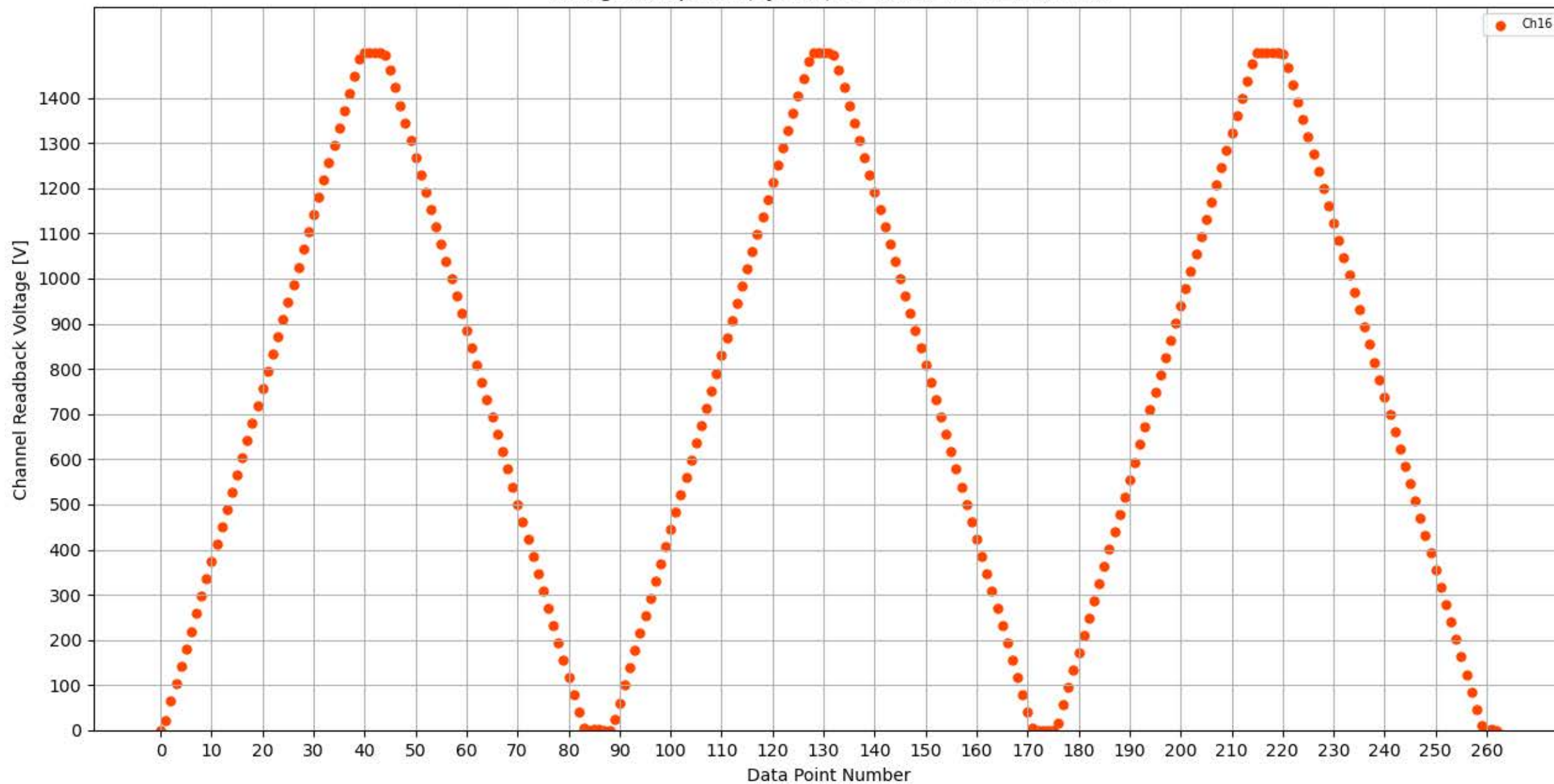
Voltage Ramp Test (Python) Bd #302, Slot #4, Ch #16
