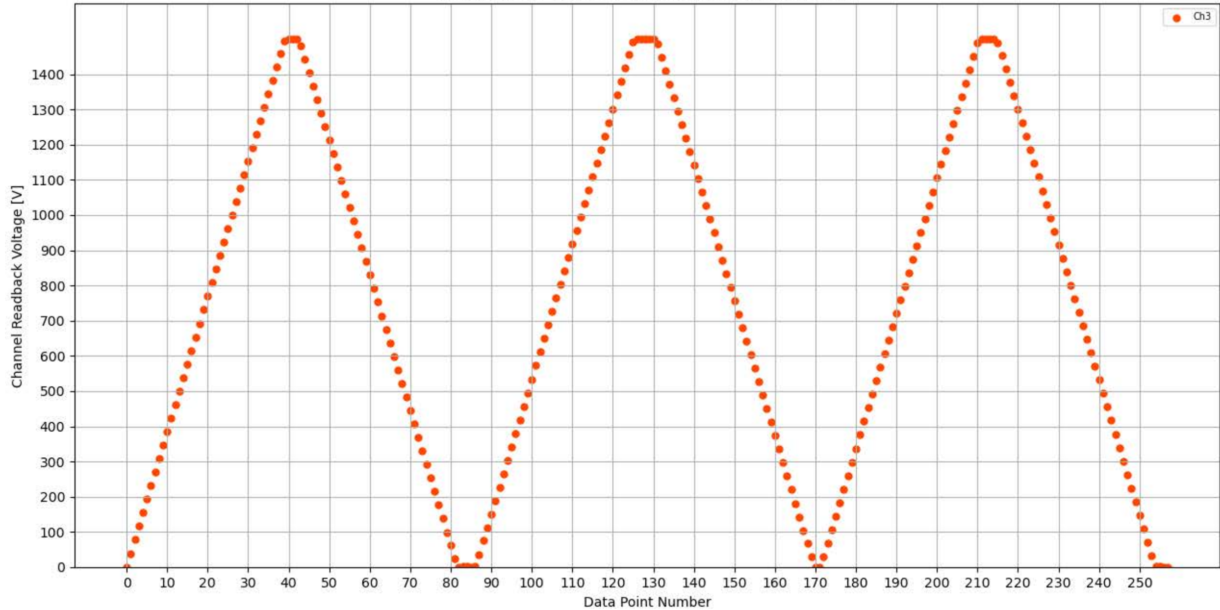
Voltage Ramp Test (Python) Bd #302, Slot #4, Ch #3
