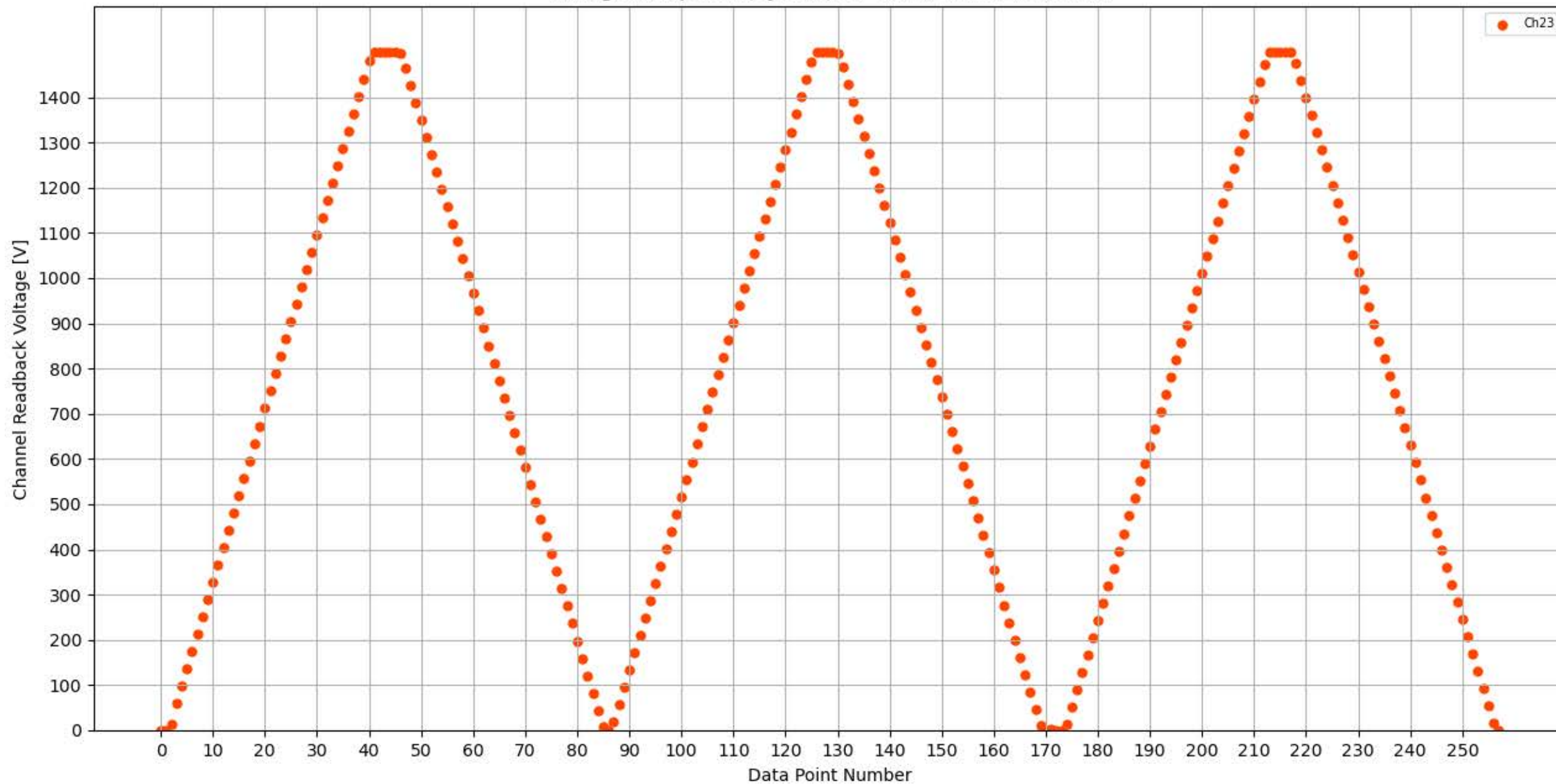
Voltage Ramp Test (Python) Bd #302, Slot #4, Ch #23
