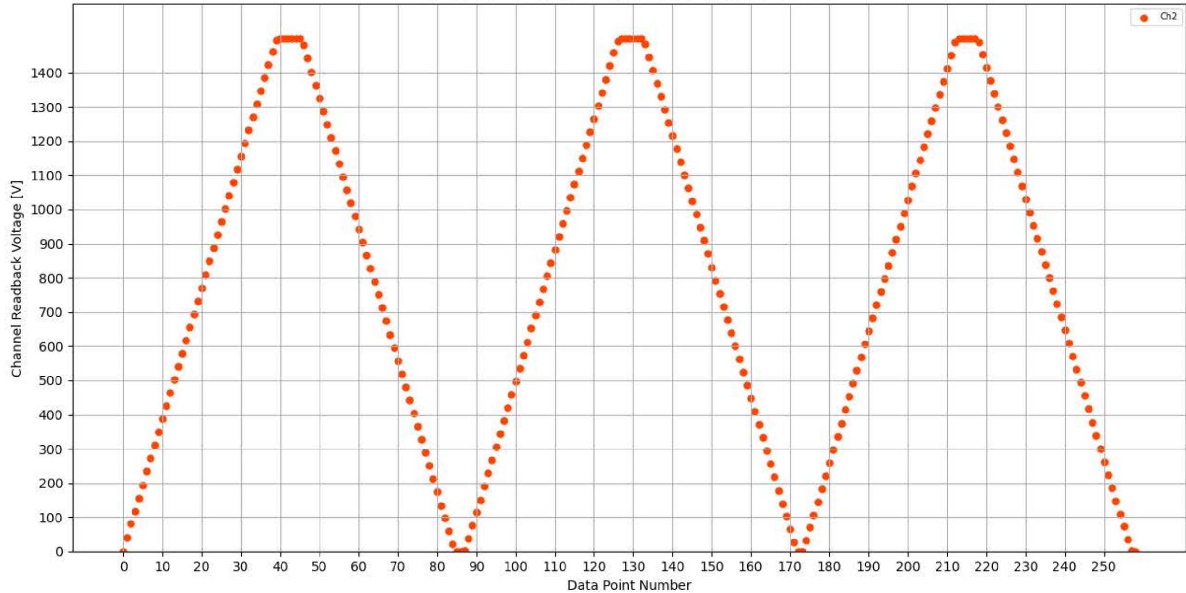
Voltage Ramp Test (Python) Bd #302, Slot #4, Ch #2
