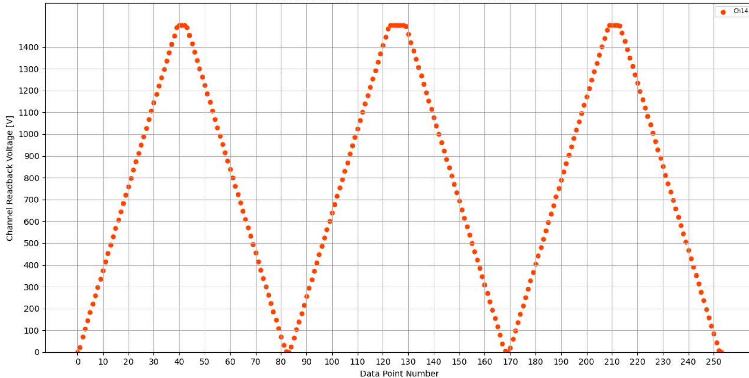
Voltage Ramp Test (Python) Bd #302, Slot #4, Ch #14
