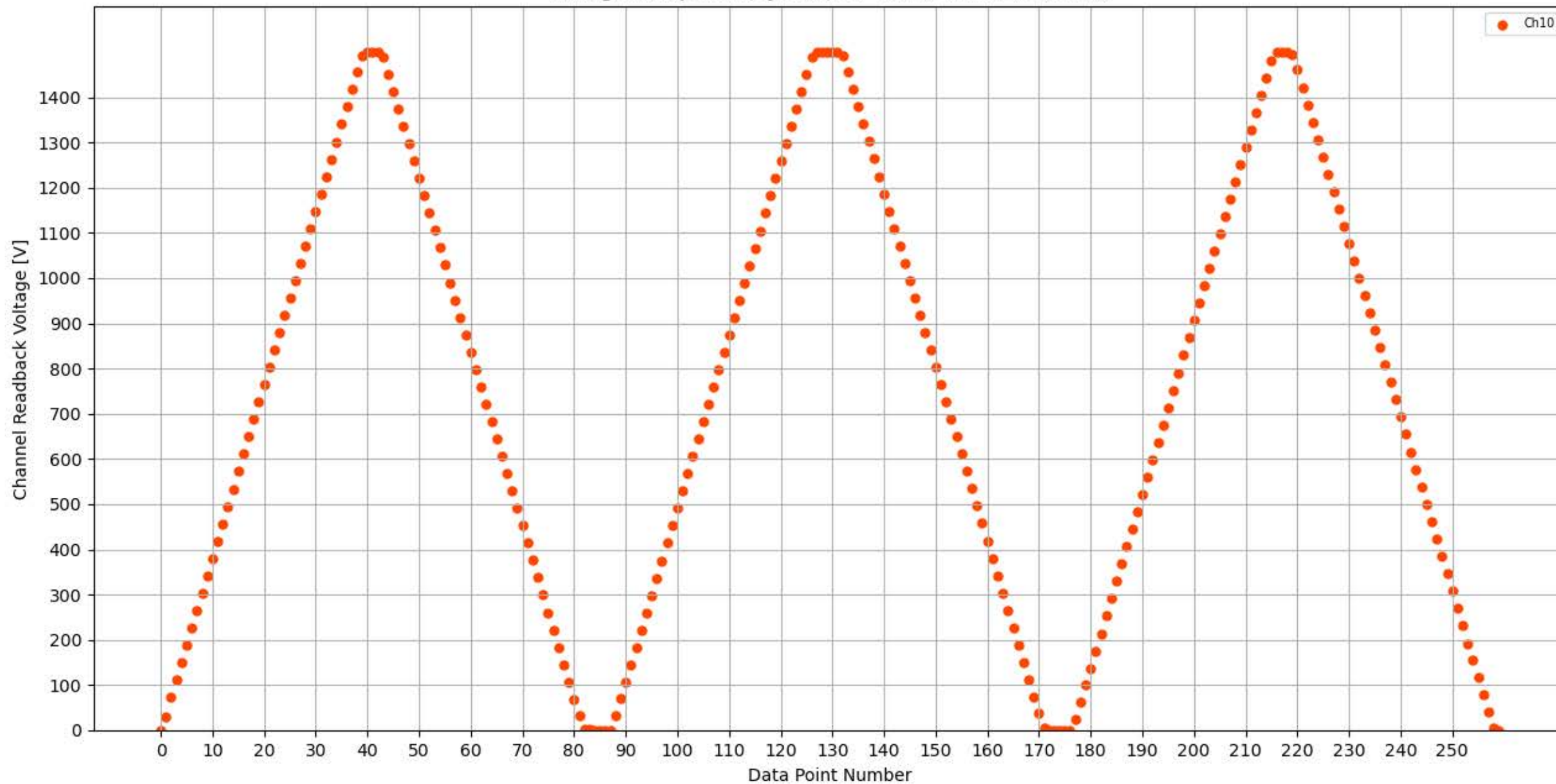
Voltage Ramp Test (Python) Bd #302, Slot #4, Ch #10
