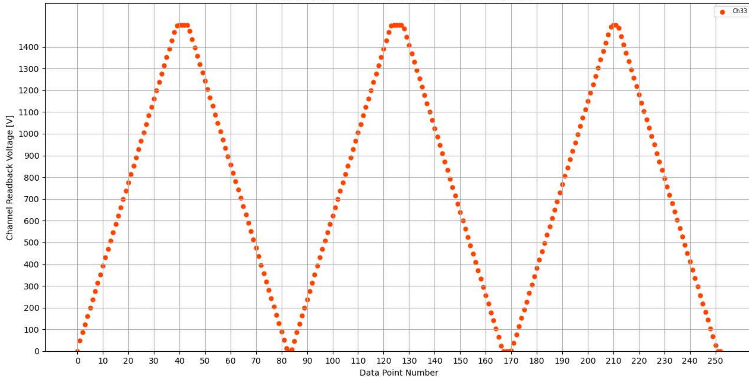
Voltage Ramp Test (Python) Bd #302, Slot #4, Ch #33
