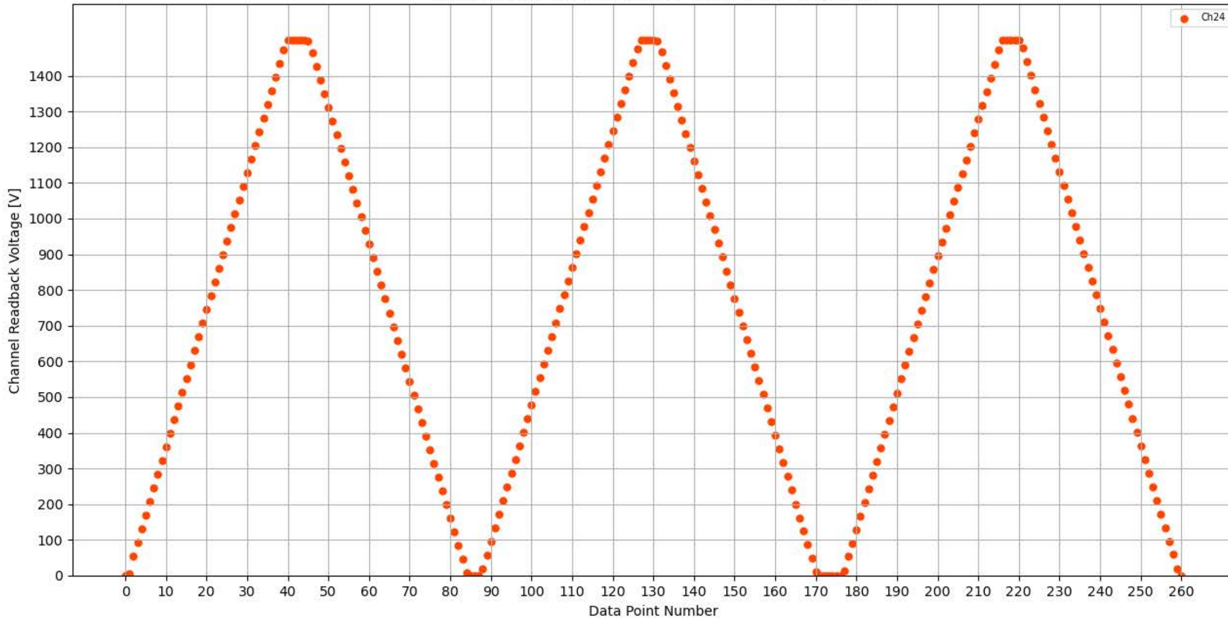
Voltage Ramp Test (Python) Bd #302, Slot #4, Ch #24
