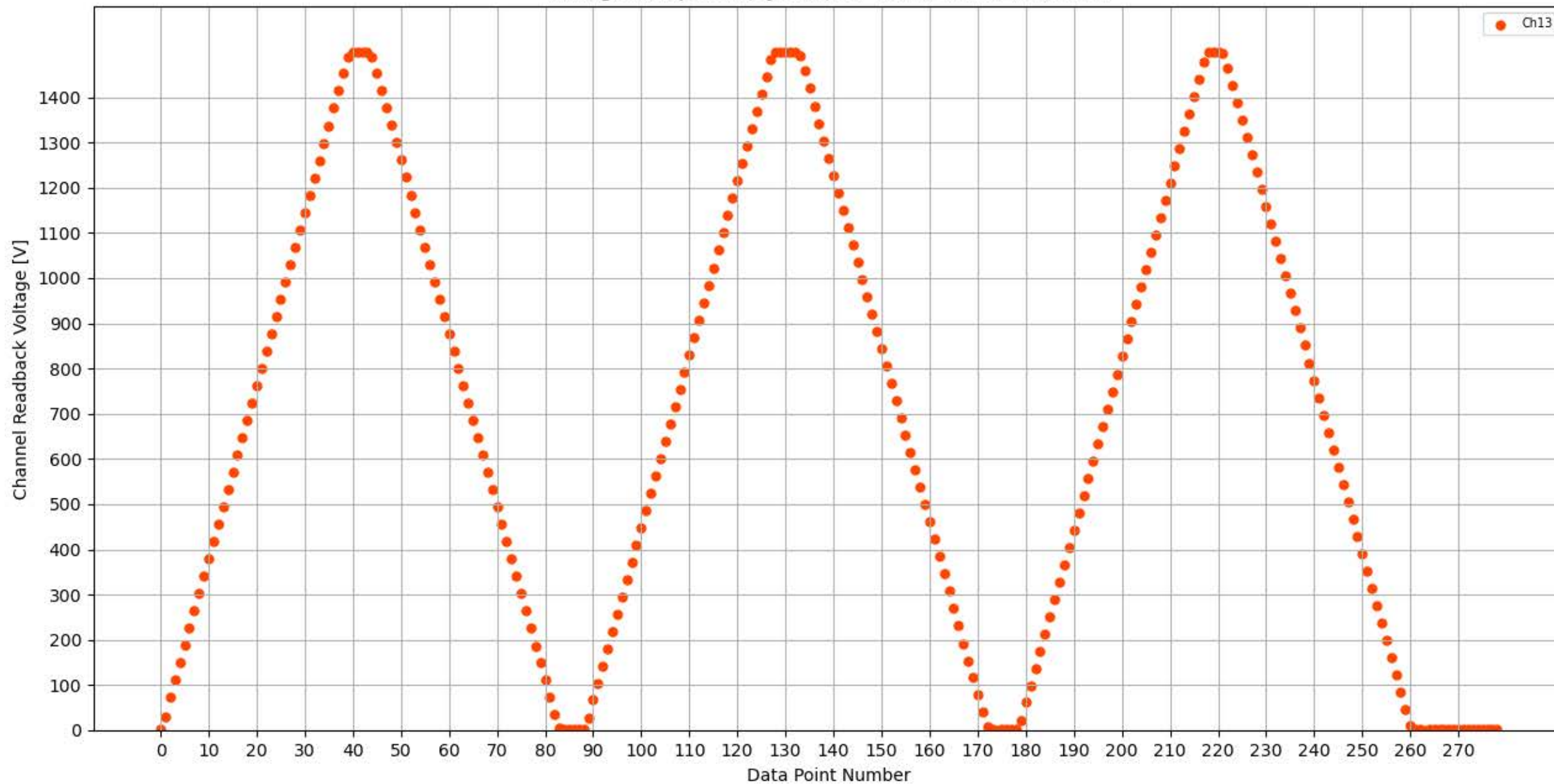
Voltage Ramp Test (Python) Bd #302, Slot #4, Ch #13
