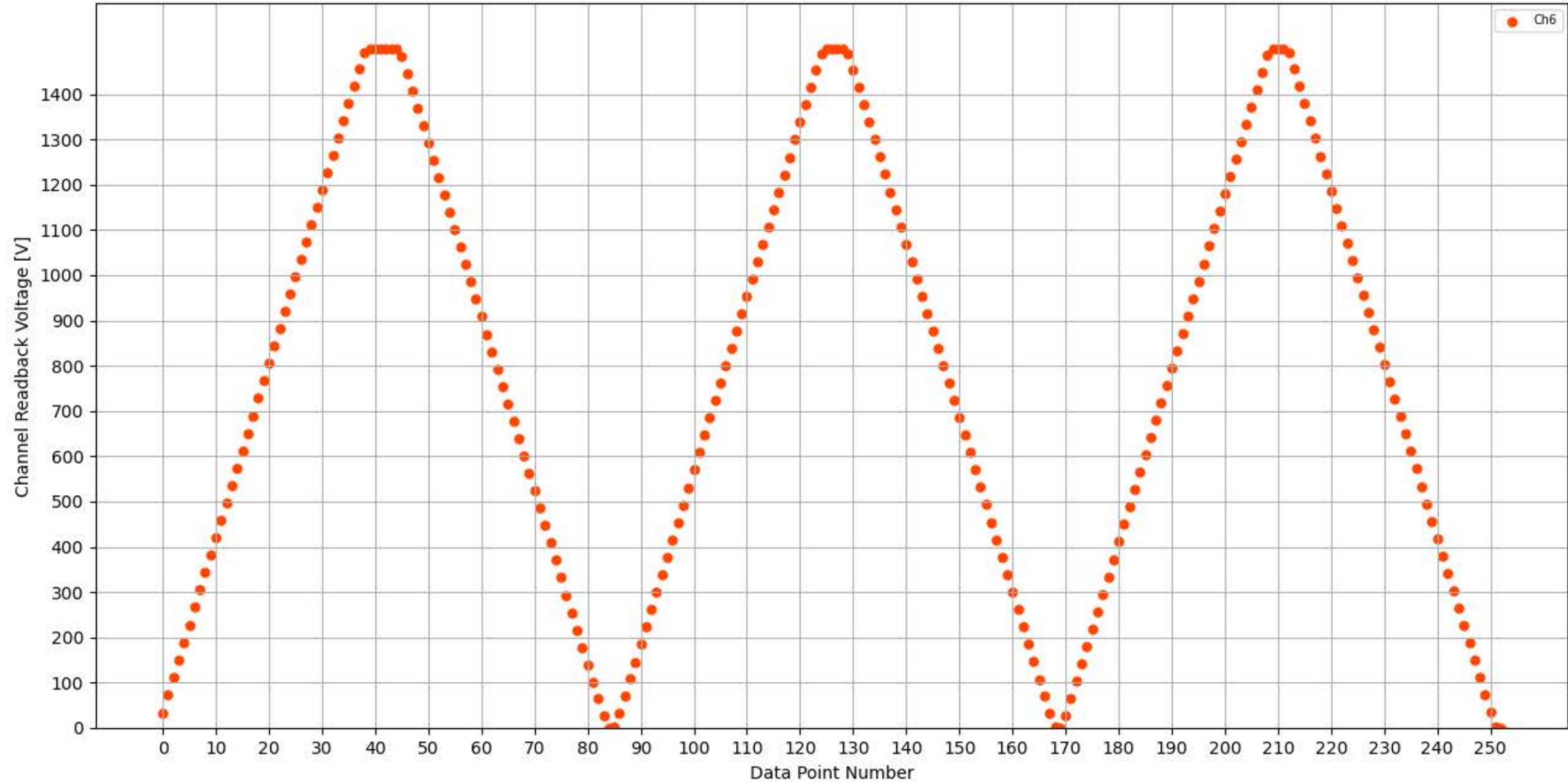
Voltage Ramp Test (Python) Bd #302, Slot #4, Ch #6
