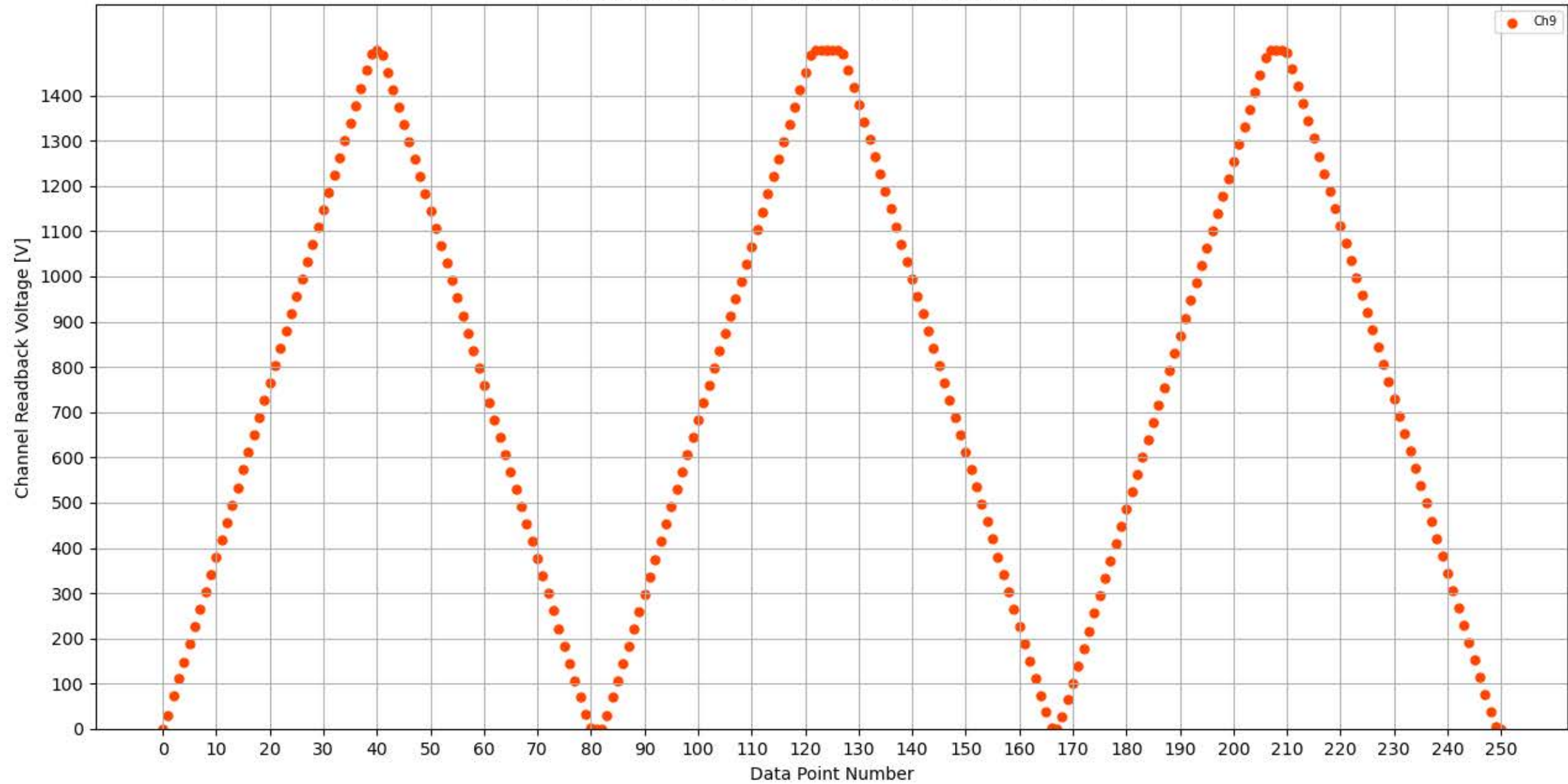
Voltage Ramp Test (Python) Bd #302, Slot #4, Ch #9
