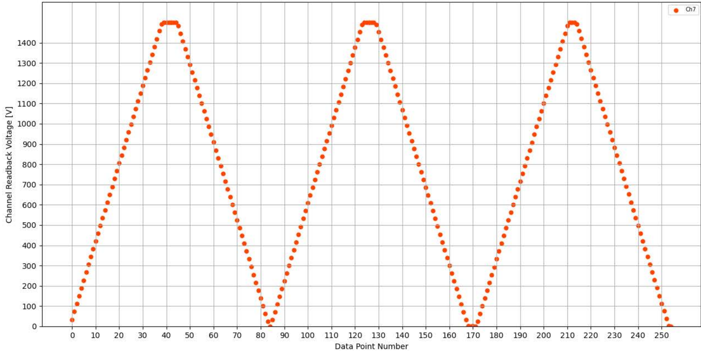
Voltage Ramp Test (Python) Bd #302, Slot #4, Ch #7
