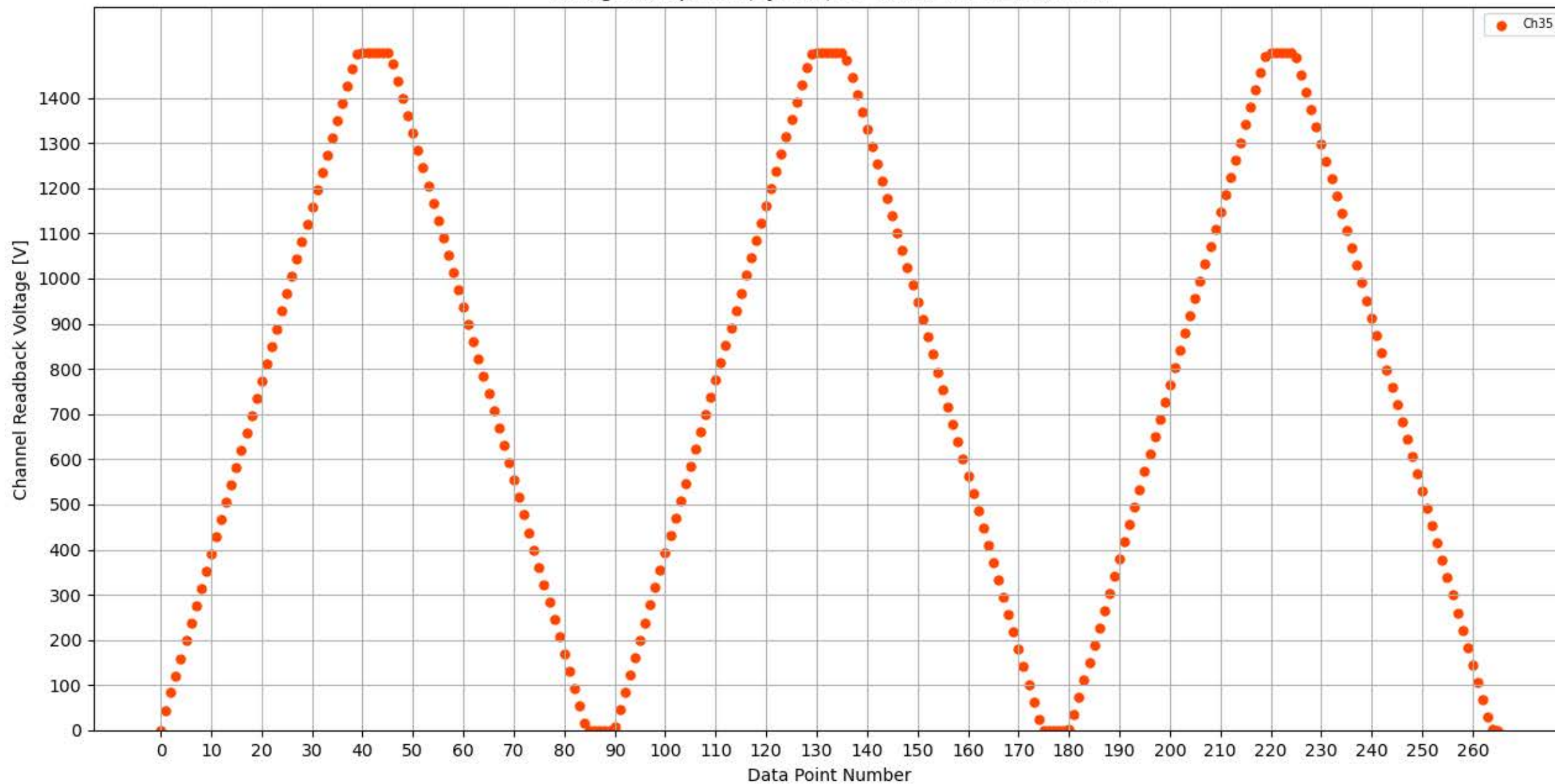
Voltage Ramp Test (Python) Bd #302, Slot #4, Ch #35
