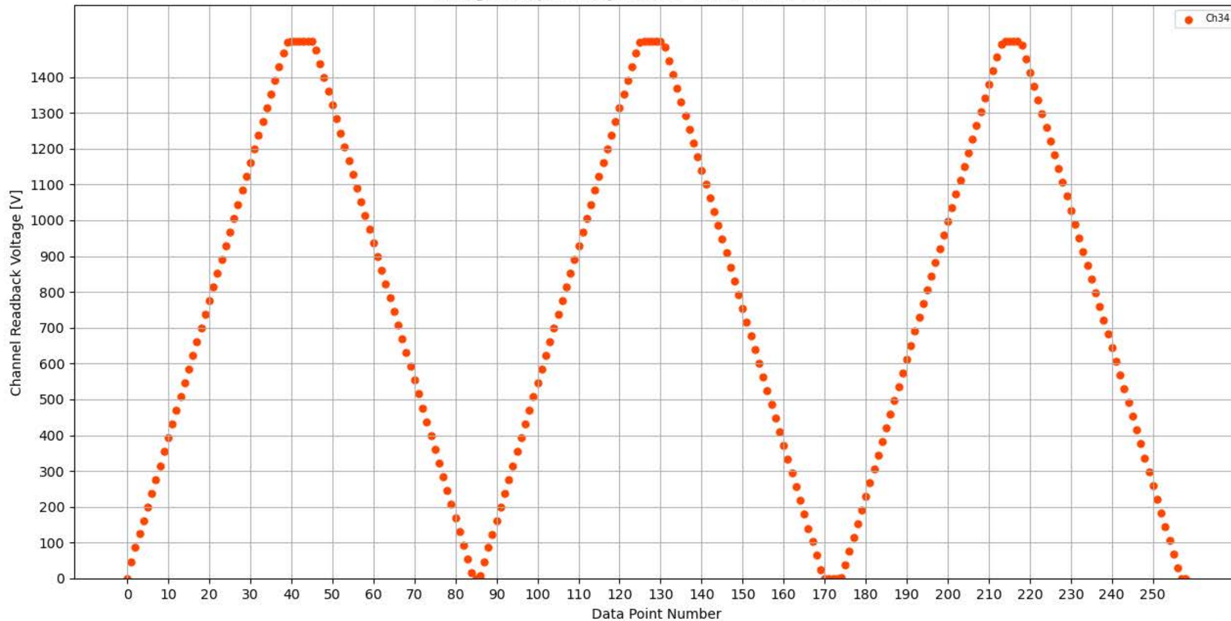
Voltage Ramp Test (Python) Bd #302, Slot #4, Ch #34
