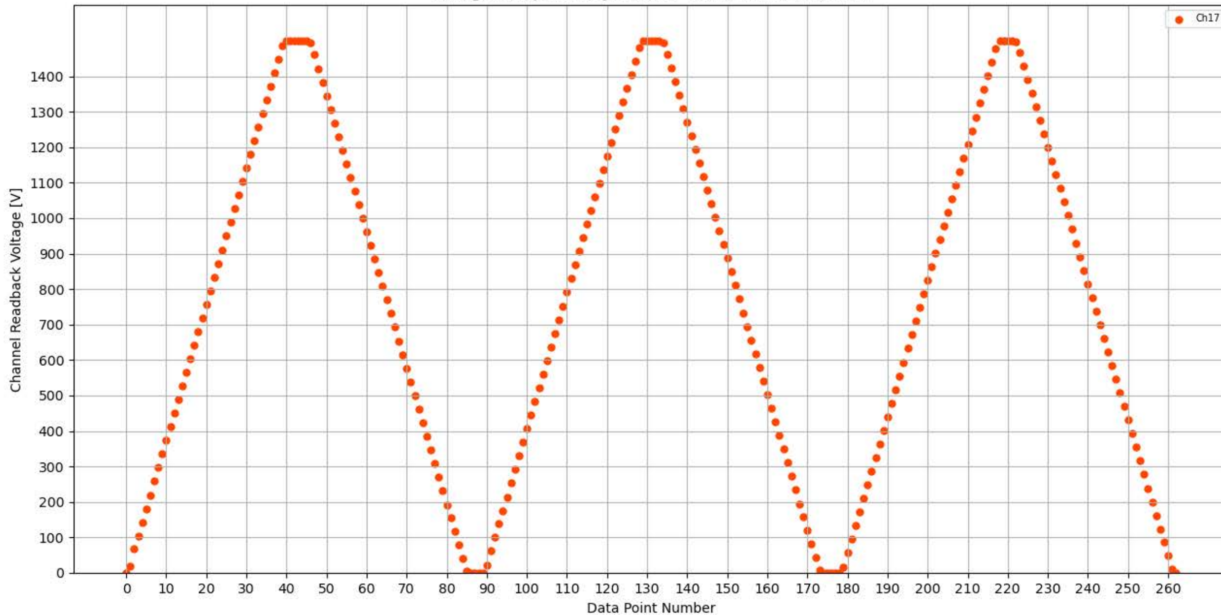
Voltage Ramp Test (Python) Bd #302, Slot #4, Ch #17
